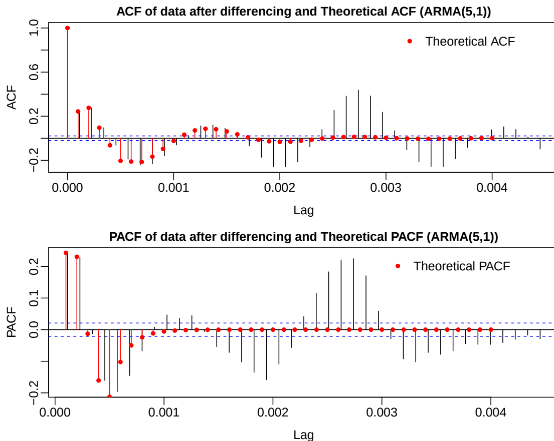
Figure 4: Comparison of ACF and PACF of data after differencing and theoretical ACF and PACF in the ARMA(5,1) model
