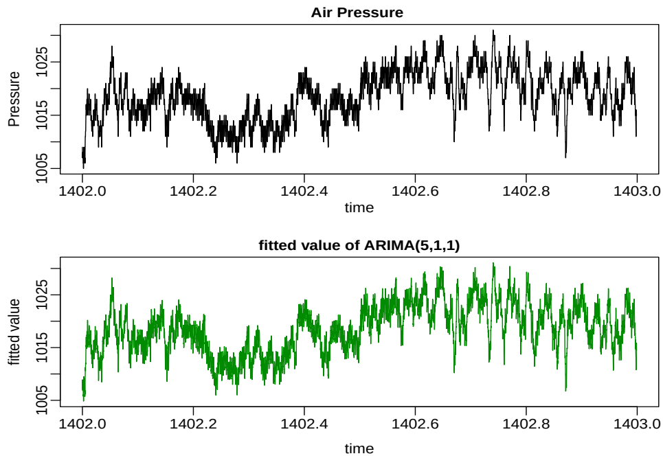
Figure 5: Time series plot of air pressure data and fitted value with ARIMA(5, 1, 1)
