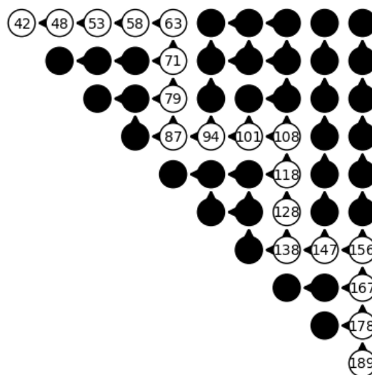
Figure 1: Backwards path witnessing (16, 16, 189^+)_{5,2} \sqsupseteq (7, 7, 42^+)_{5,2} .
