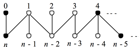
Figure 1: Rosa’s \alpha -labeling scheme for a caterpillar
